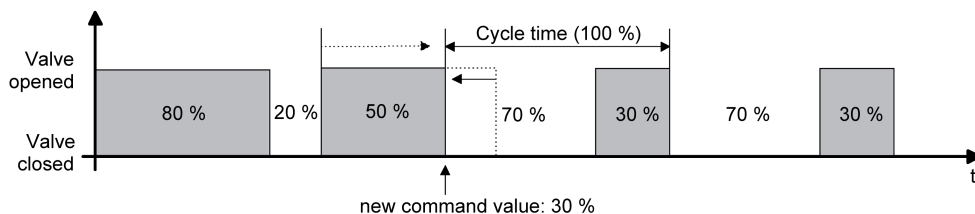
Figure 12: Example of a command value change 80 % -> 30 % during the opening phase of the valve (opening phase too long)
