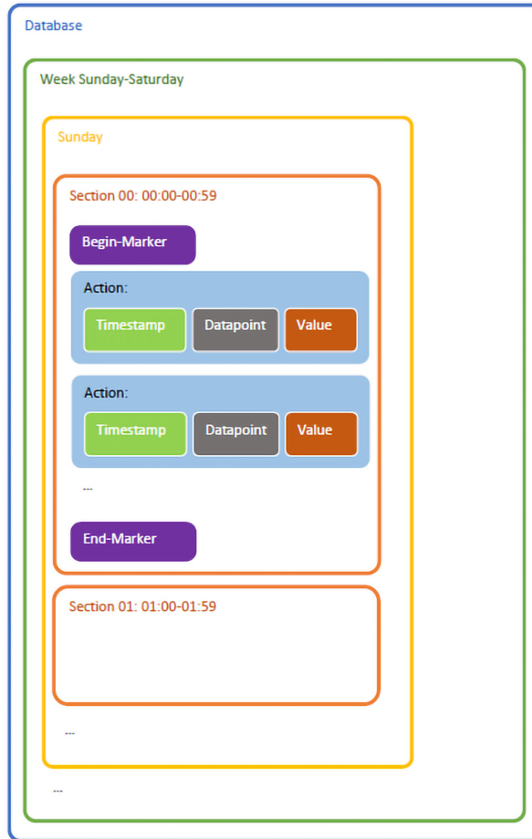
Fig. 71: JUNG Smart Vision – Diagram of the data structure of the recording
