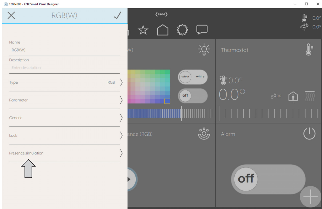
Fig. 49: Smart Panel Designer – Adding elements to a presence simulation
