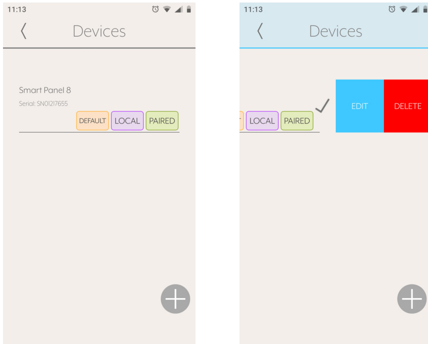
Fig. 79: JUNG Smart Vision – Paired device in the “Devices” menu and editing the device (client)
