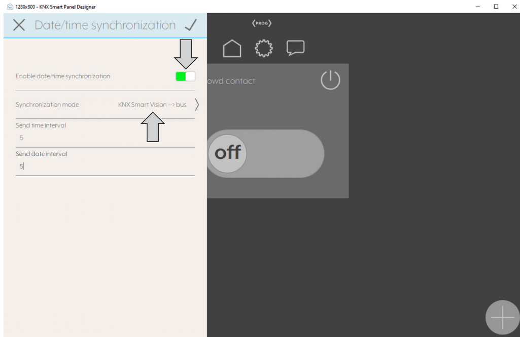
Fig. 47: Smart Panel Designer – “Synchronise date/time” submenu
