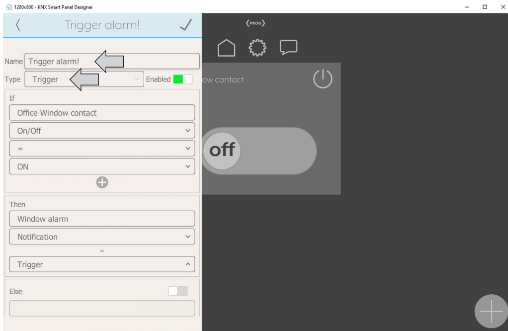
Fig. 38: Smart Panel Designer – “New logic operation” submenu
