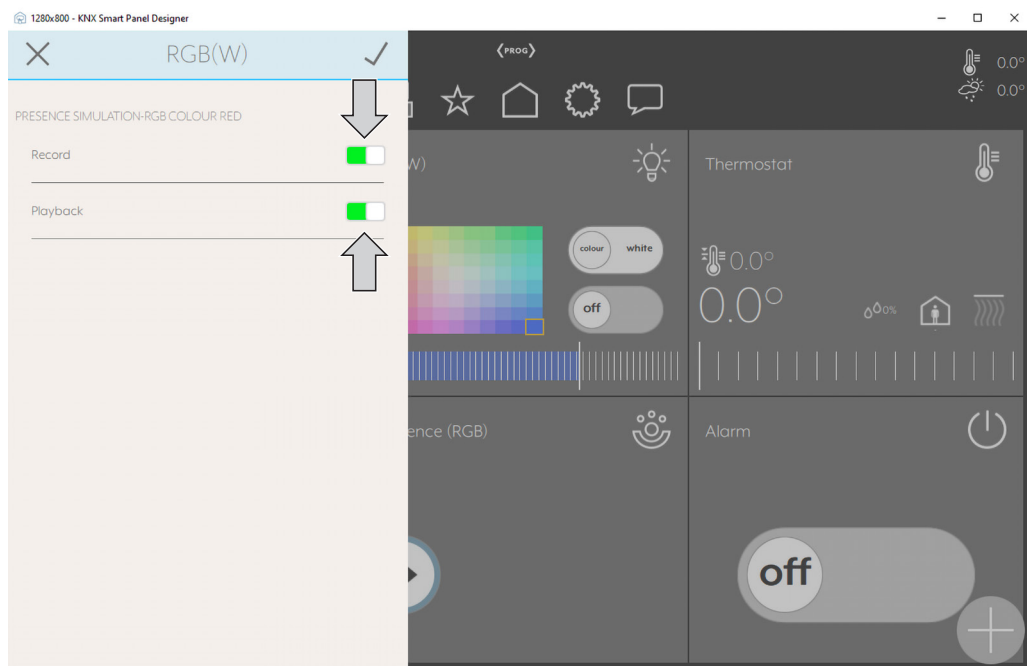
Fig. 51: Smart Panel Designer – Recording and playback of the element for presence simulation
