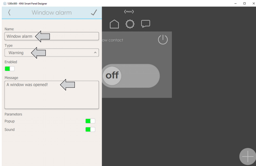
Fig. 40: Smart Panel Designer – “New messages” submenu
