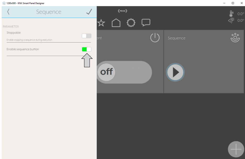
Fig. 53: Smart Panel Designer – Activating the sequence push-button for an element
