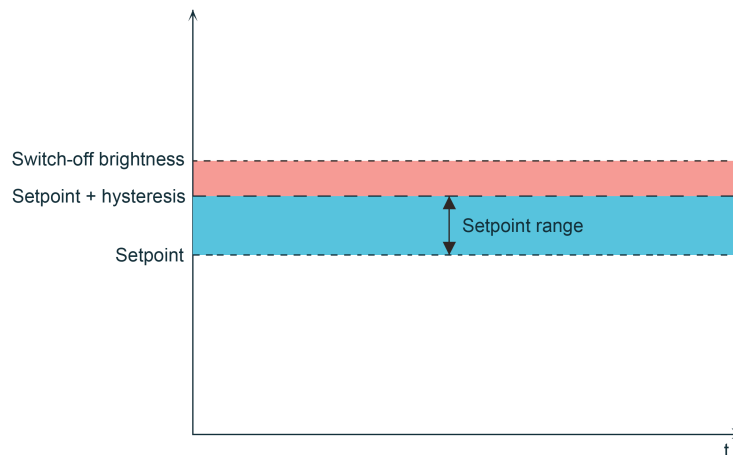
Figure 57: The switch-off brightness results relatively from the setpoint and hysteresis value of the setpoint
